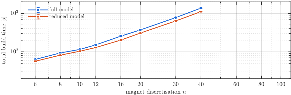
Iteration 1: inline field, -O2 compile
